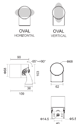
Physical Dimension(MM)
