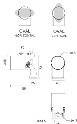
Physical Dimension(MM)
